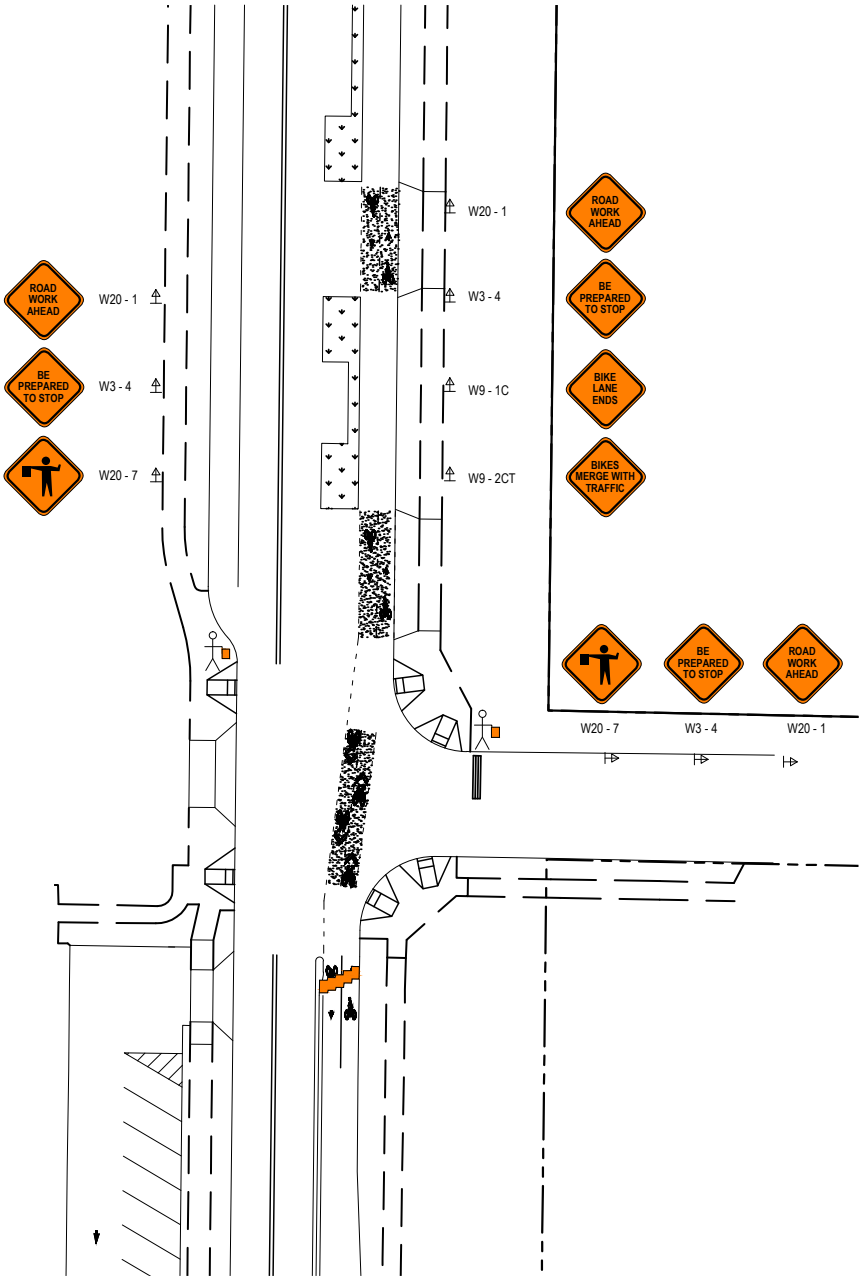
PROTECTED BIKE LANE CLOSURE - FAR SIDE LANE
