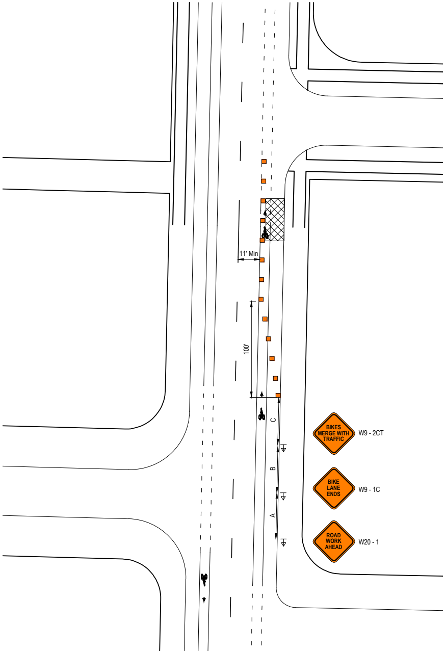
BIKE LANE CLOSURE TYPICAL DIMENSIONS OF A, B, & C
