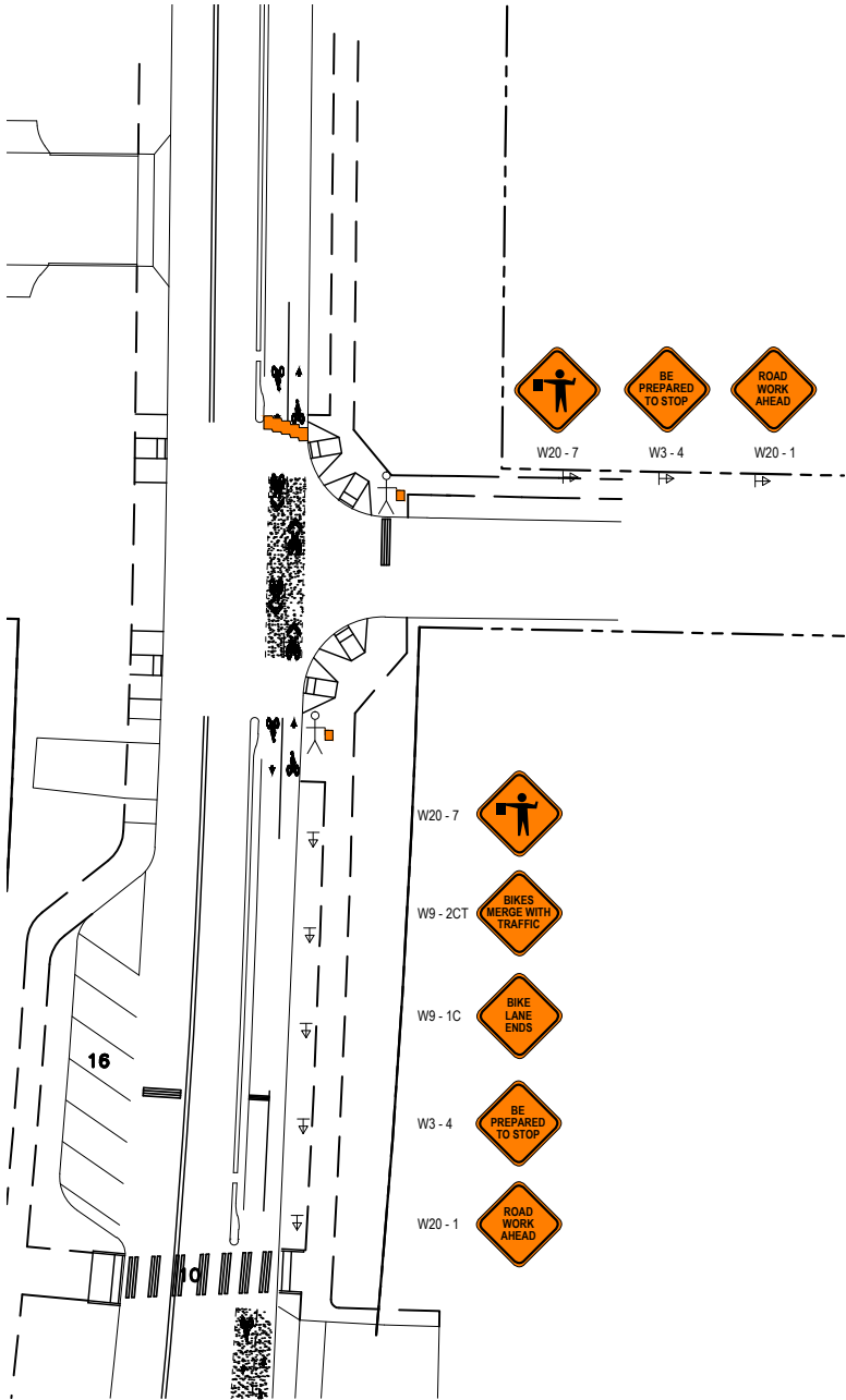
PROTECTED BIKE LANE CLOSURE - NEAR SIDE LANE
